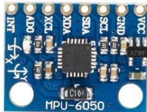
Figure 1. MPU-6050 sensor module [8]
