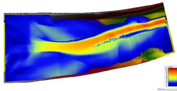
Figure 3. Velocity values of 2D modeling
