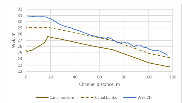
Figure 5. Longitudinal profile of the stilling basin and tailrace canal
